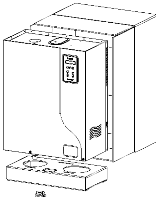
Fig. 2-1. Steam Generator ElectroVap® STEAM BATH
