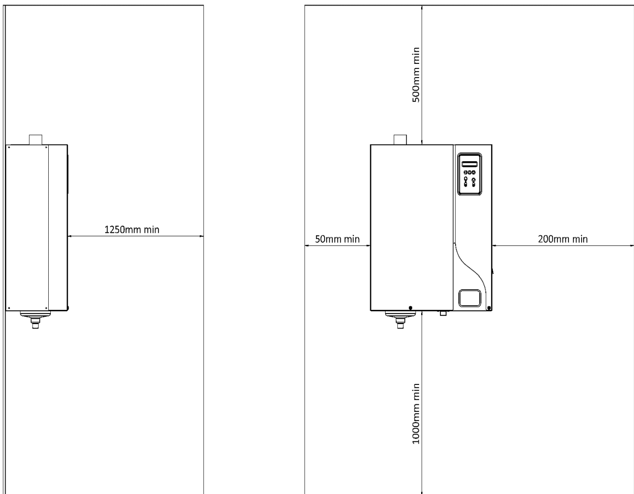
Fig.2-4. Mounting distances
