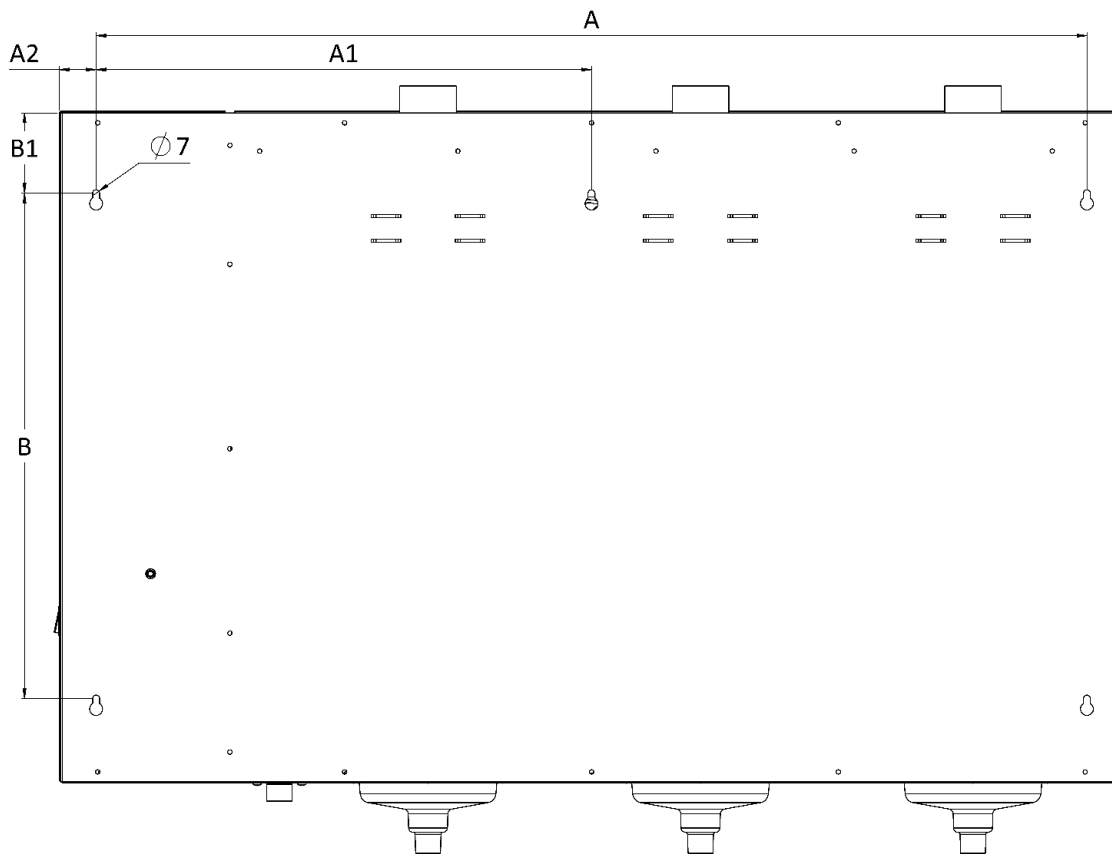
Fig. 3-1. Installation holes
